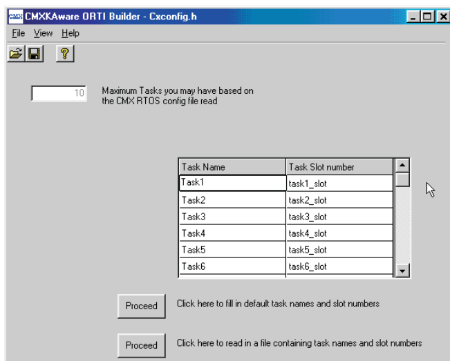
CMX-KAware ORTI Builder
