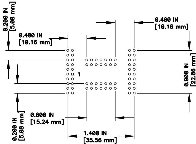
Target POD Pinout –Dimensions
