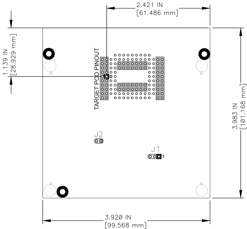
Motorola 68EC000 ActivePOD, bottom view
