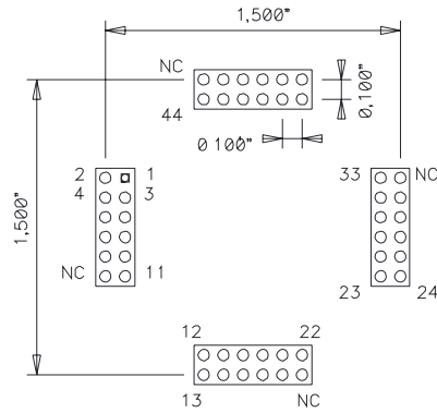
Target POD Pinout
