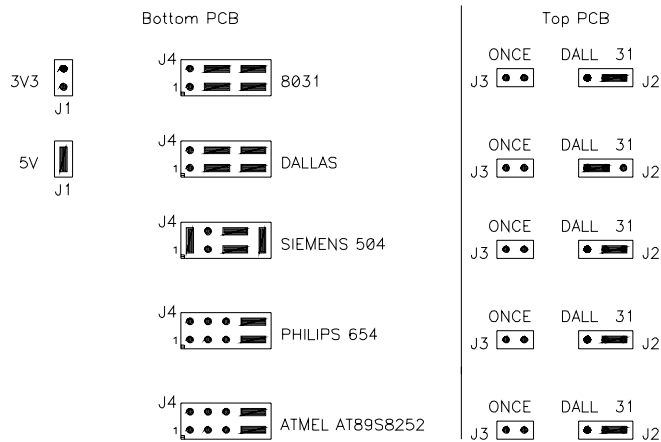
Jumper settings for CPU types
