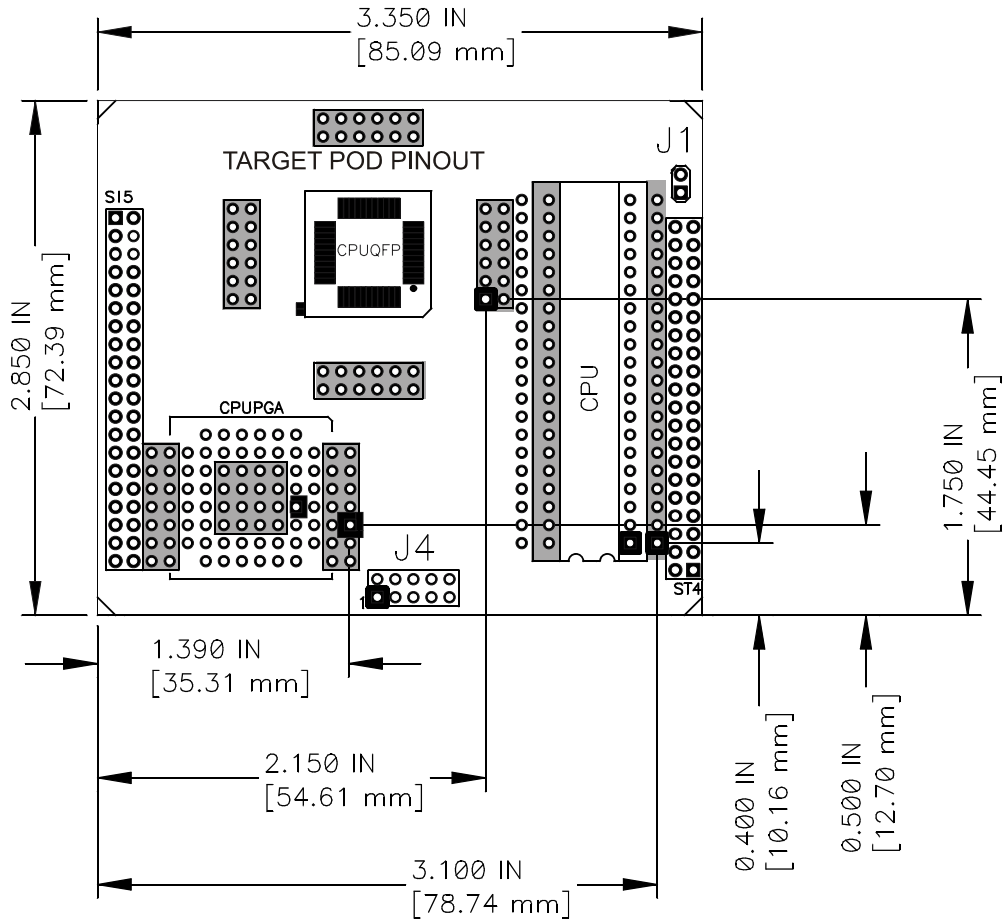
Bottom board
