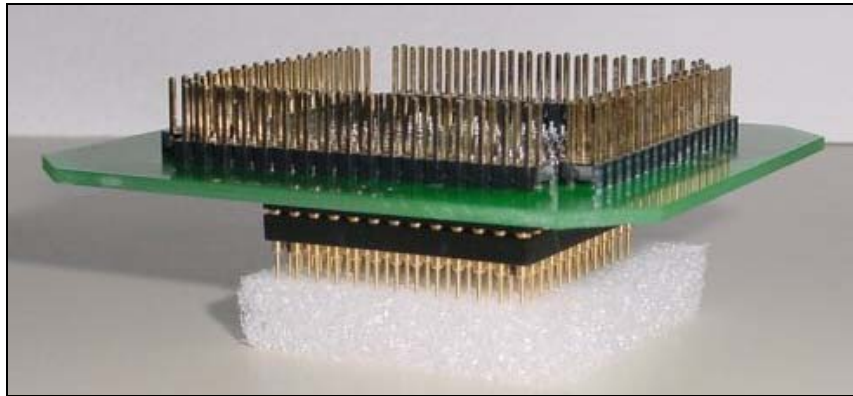
IA132PODPGA adapter
