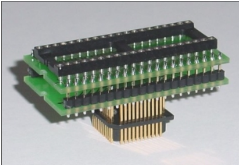
IA40D44P8031 adapter
