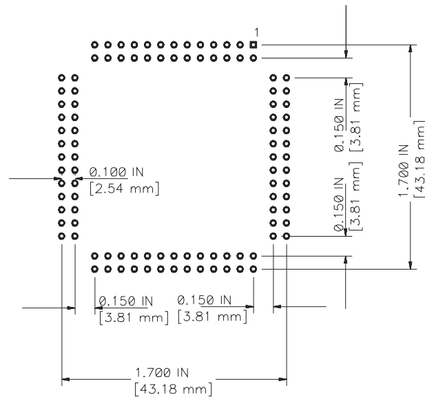
T_QFP100S Pinout Dimensions
