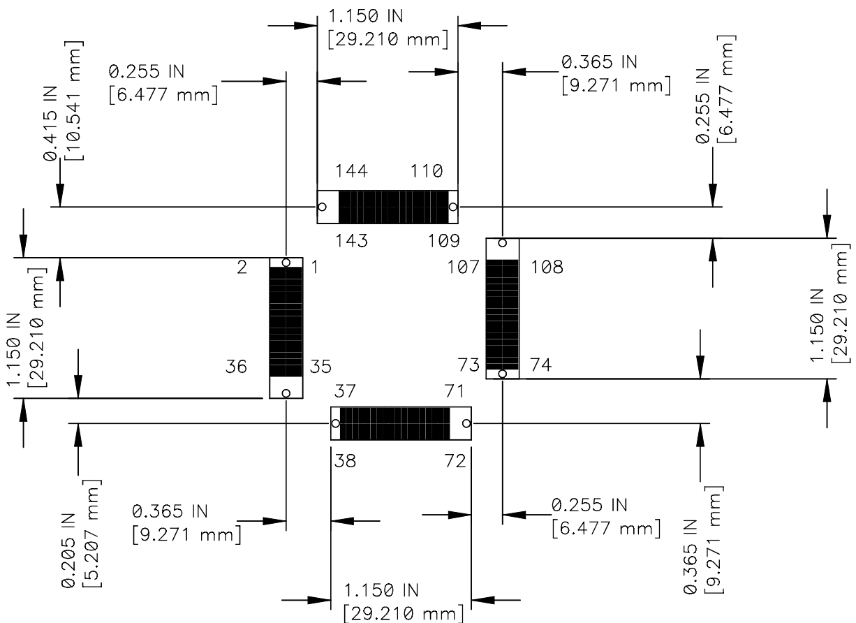
T_QFP144 – Dimensions
