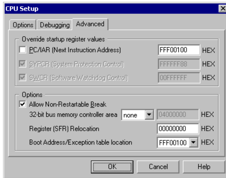
PowerPC Family Advanced Options
