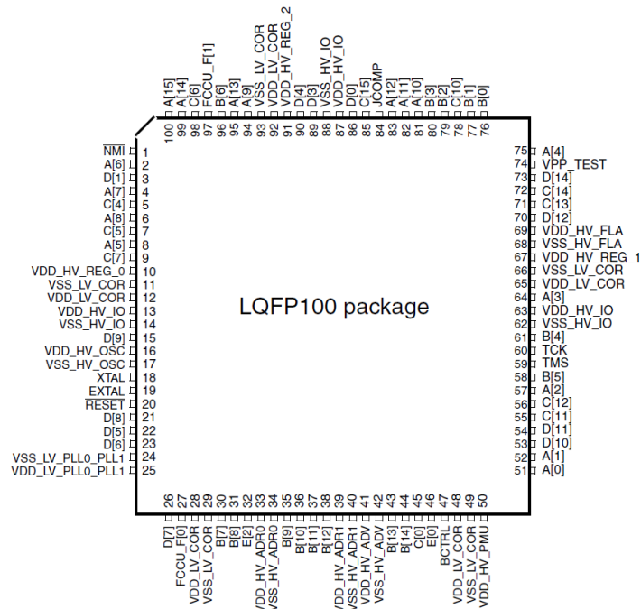
Target microcontroller SPC56EL70 – 100 LQFP pin configuration
