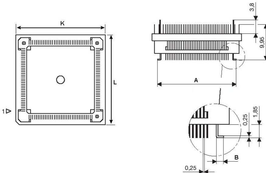
IA100TQ-SOLDER dimensions
