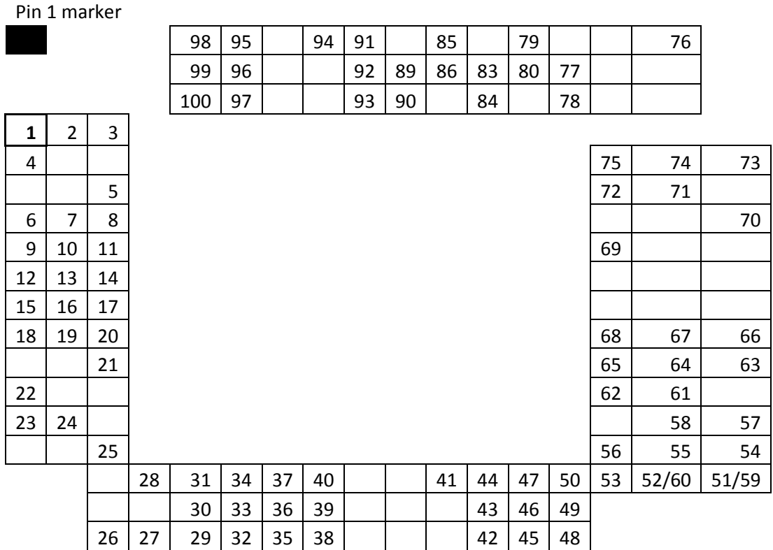
100-pin layout – emulation adapter top view
