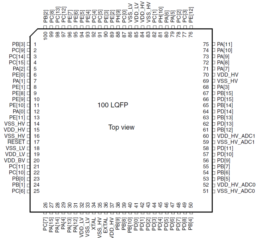
Target microcontroller MPC5607B – 100 LQFP pin configuration
