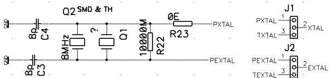
Crystal circuit
