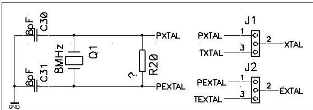
Crystal circuit
